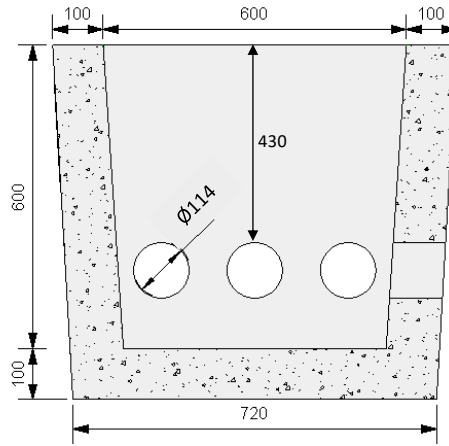
SIDE ELEVATION
